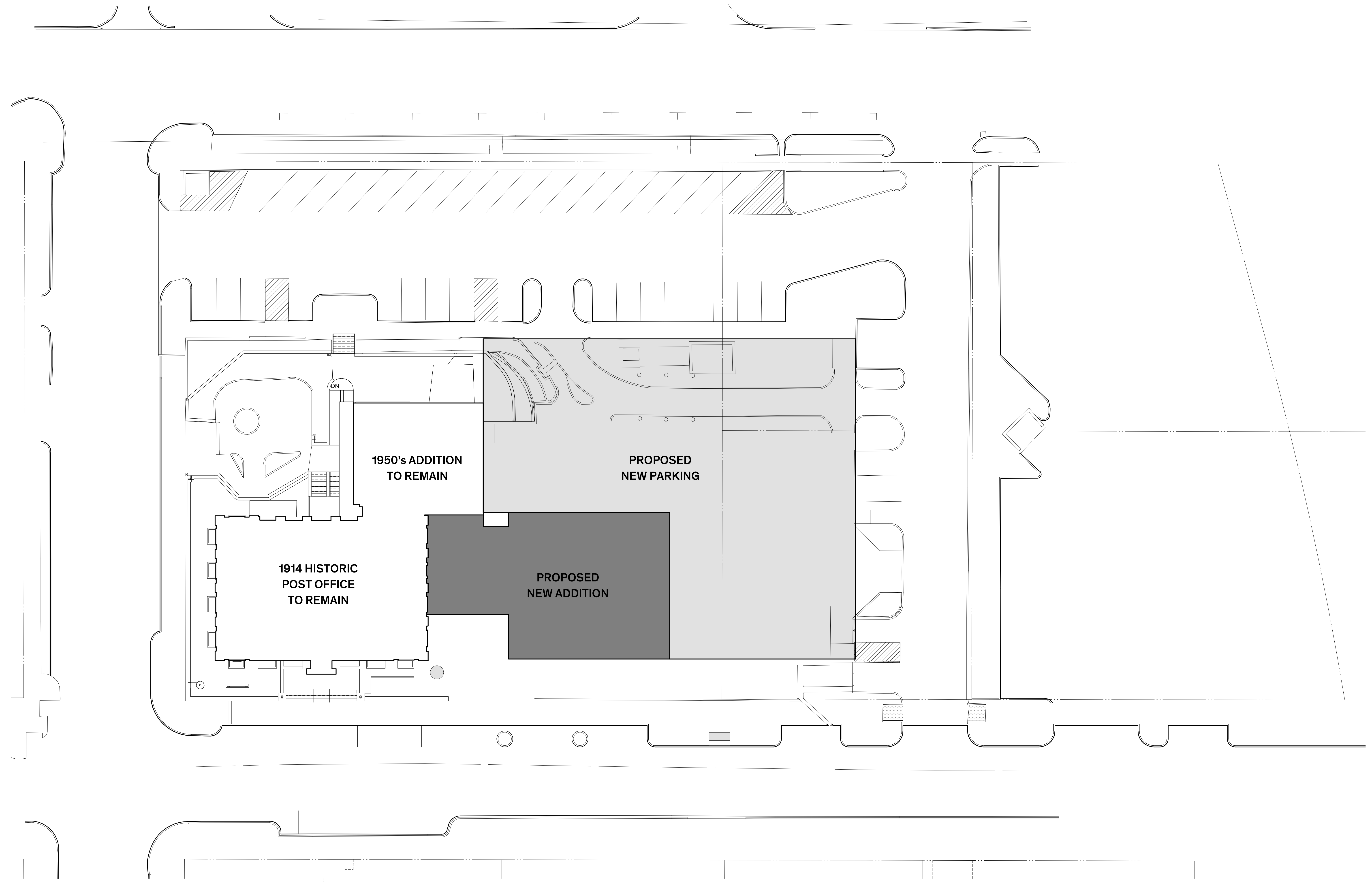
1 Site Plan 1/16" = 1'-0"
